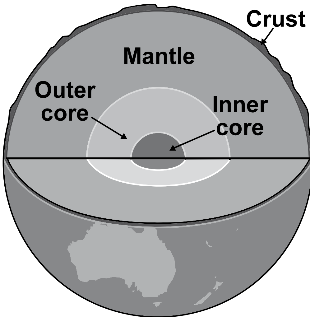
Cutaway diagram of the Earth
